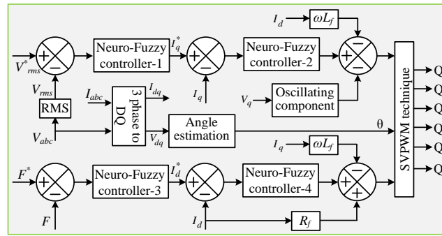
Fig. 4: Neuro-Fuzzy controller based proposed inverter controller
