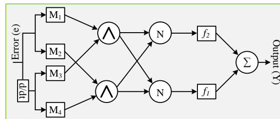
Fig. 2: Neuro-Fuzzy system model.
