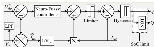
Fig. 3: Proposed control method of dc circuit.
