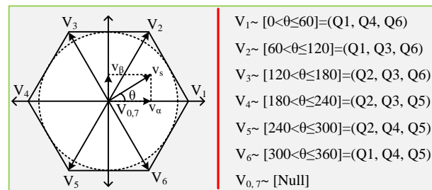
Fig. 5: SVPWM Technique
