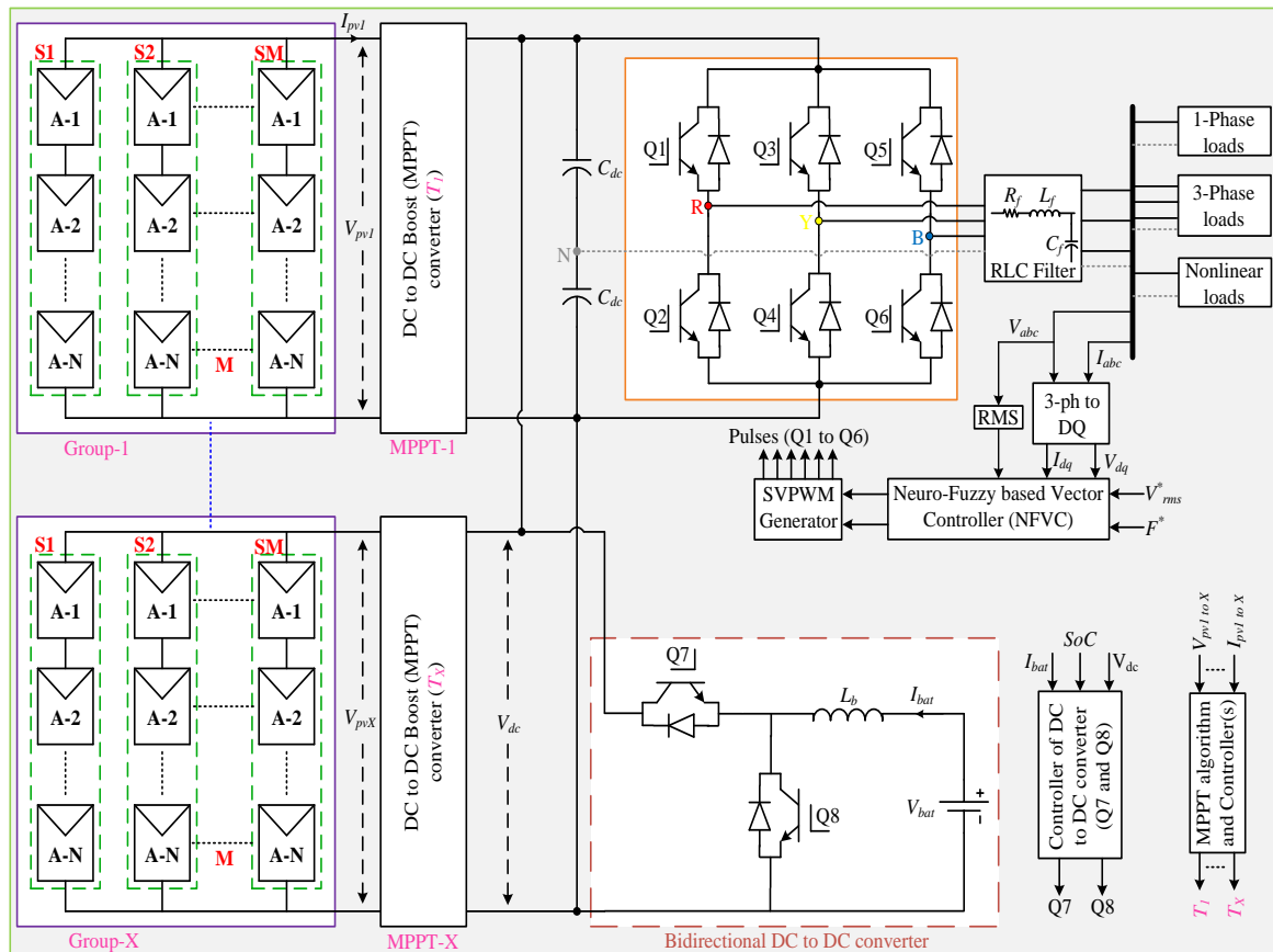
Fig. 1: A standalone model.
