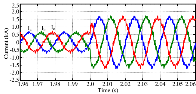
Fig. 9: Instantaneous currents at PCC.
