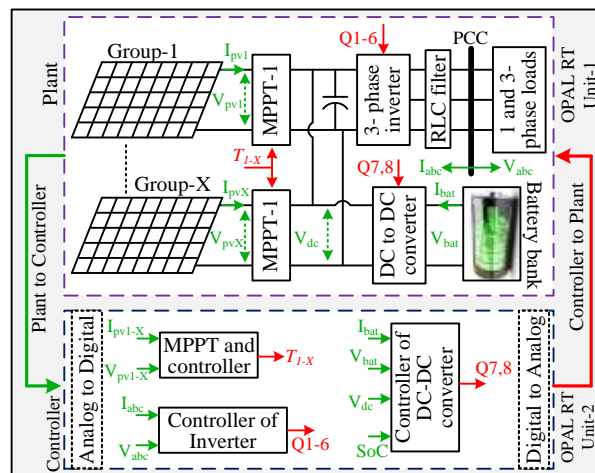
Fig. 7: Model HIL block of proposed system.
