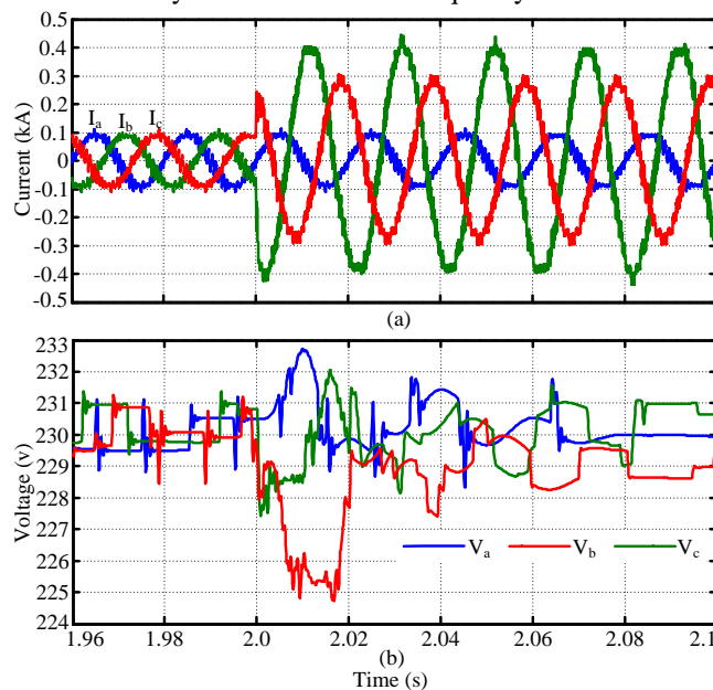
Fig. 10: (a) Load current, (b) voltages.
