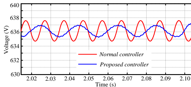
Fig. 11: second frequency oscillations in dc-link
