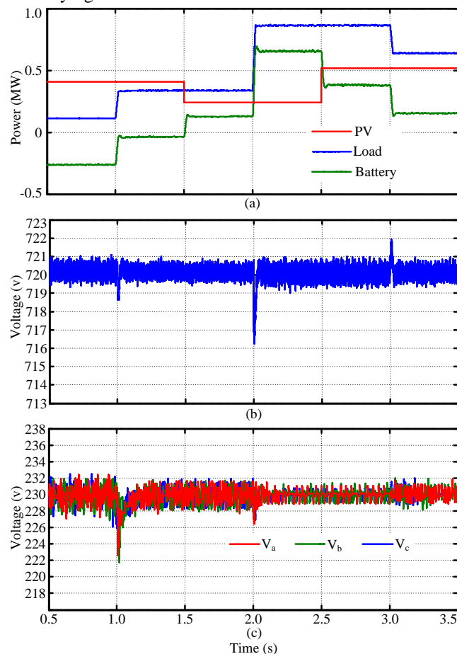
Fig. 8: (a) Powers, (b) dc-link, (c) RMS voltage
