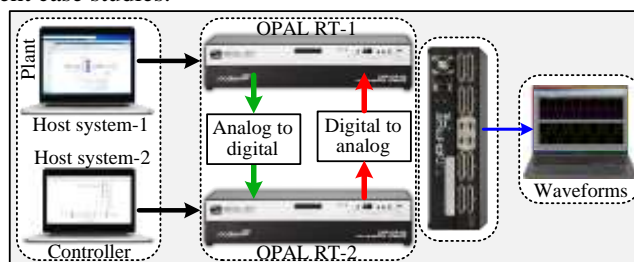
Fig. 6: HIL configuration.
