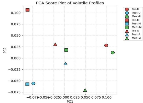
Figure 12: PCA score plot for volatile compound profiles across all formulations and treatments.
